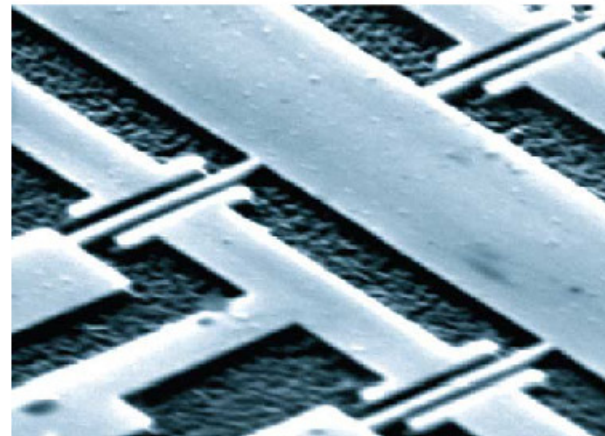
Figure 1 | Hang in there. A scanning electron micrograph of a set of suspended silicon nanomechanical beams with electrostatic control gates. Each beam can be made to move between two buckled states (0 or 1) by applying a field to its control gates. Stochastic resonance could allow enhanced control in switching between the two discrete states, and use of these nonlinear states as nanomechanical memory cells.
